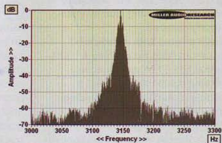
ABOVE: Wow and flutter re. 3150Hz tone at 5cm/sec (plotted ±150Hz, 5Hz per minor division). Wow is very low and flutter, though complex, is also low
