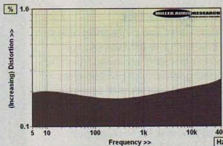
ABOVE: Distortion vs. extended frequency from 5Hz-40kHz, 10W/8ohm – moderately high, but consistent
