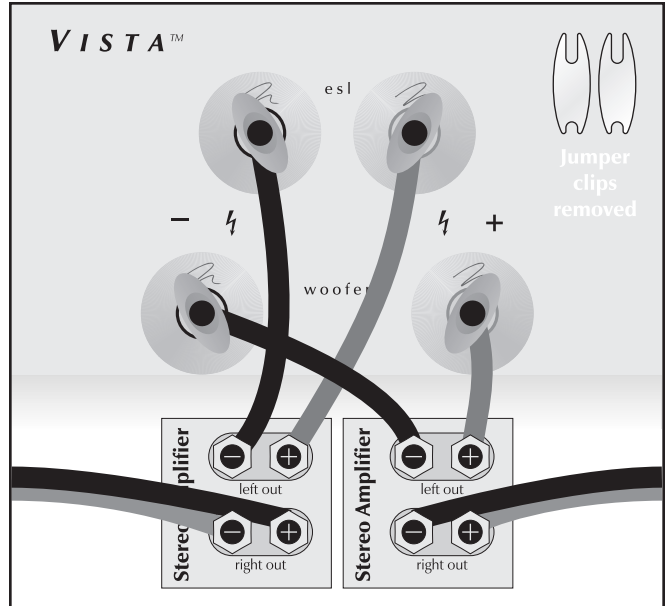
Figure 4. Horizontal bi-amplification connection. One channel shown.
