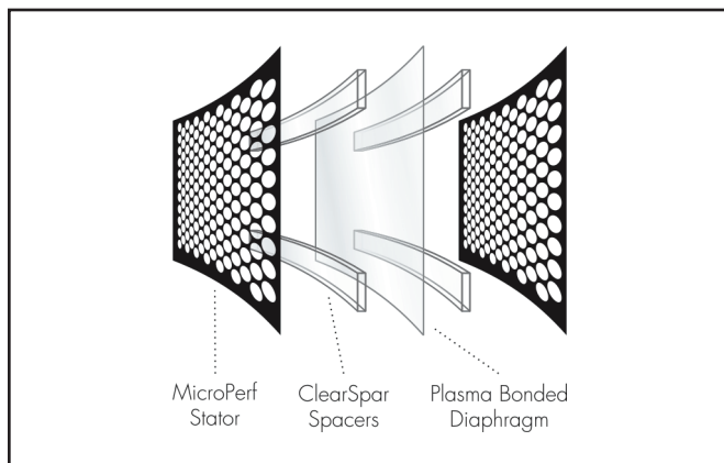
Figure 15. Cut away view of an XStat™ electrostatic transducer. Notice the simplicity due to minimal parts usage.
