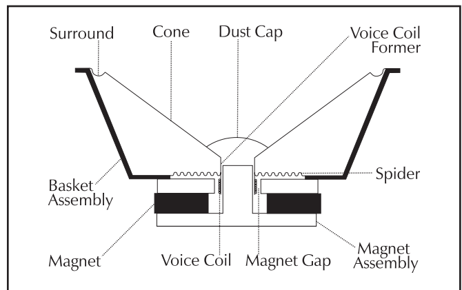
Figure 16. Cut away view of a typical moving coil driver. Notice the complexity due to the high number of parts.
