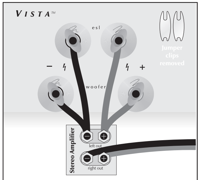
Figure 3. Bi-wire connection. One channel shown.
