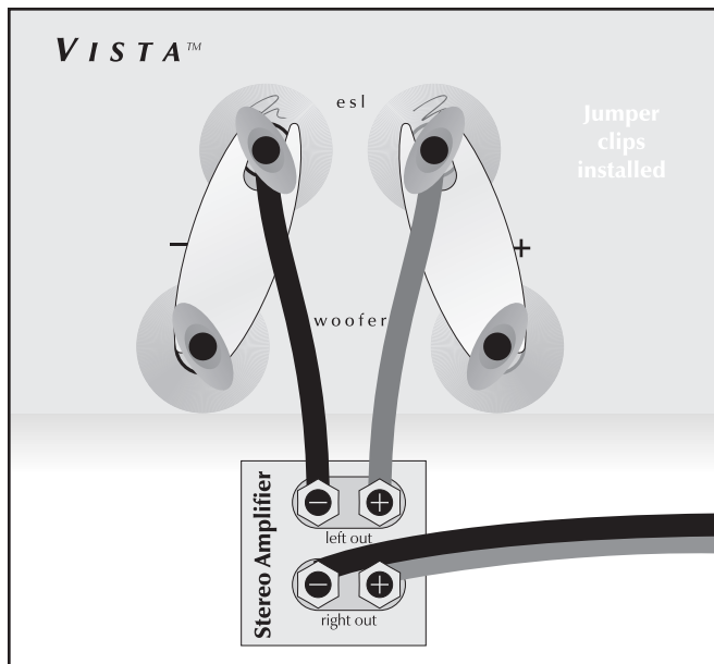
Figure 2. Single-wire connection. One channel shown.
