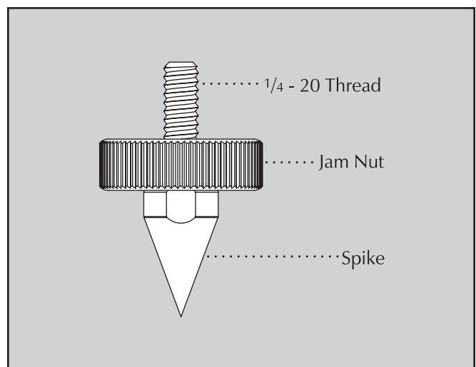
Figure 7. The ETC™ Spike.
