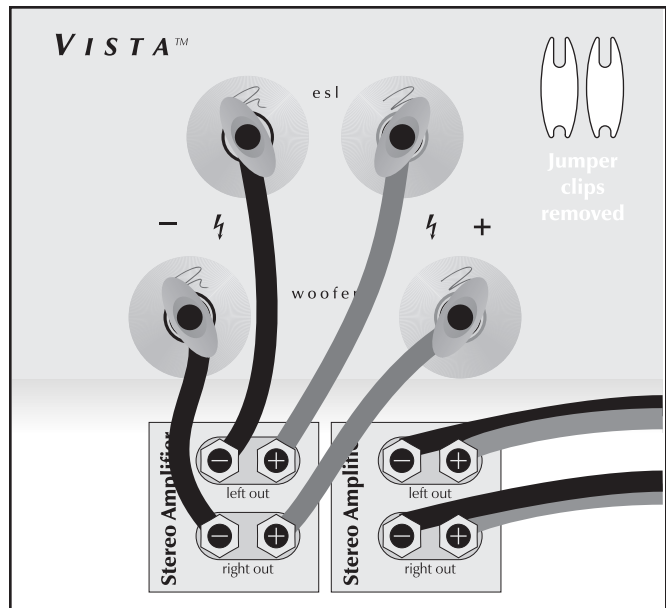
Figure 5. Vertical bi-amplification connection. One channel shown.
