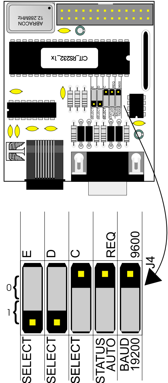
Figure 7 – Citadel RS232 Jumper Settings
