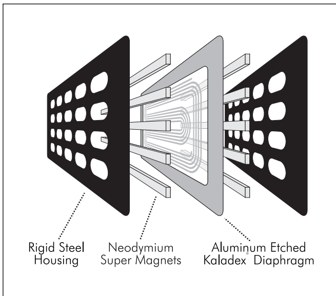
Figure 5. Cut away view of an ATF transducer. Note the simplicity due to minimal parts usage.
