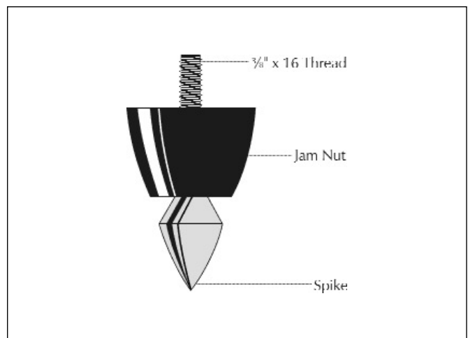
Figure 6. The ETC Spike.
