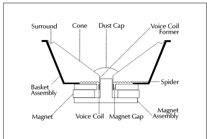
Figure 16. Cut away view of a typical moving coil driver. Notice the complexity due to the high number of parts.
