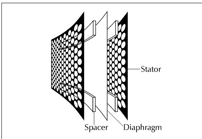
Figure 15. Cut away view of an electrostatic transducer. Notice the simplicity due to minimal parts usage.
