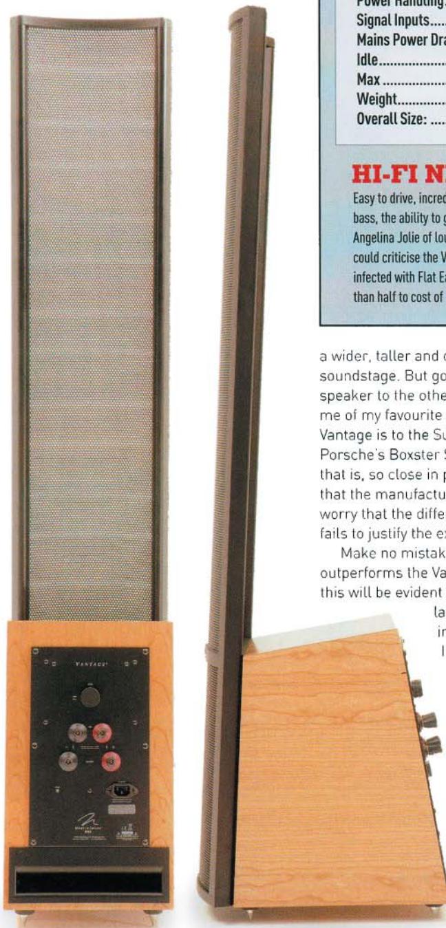
LEFT: A rotary to the rear of each bass unit allows bass output to be tailored to suit different listening environments while twin speaker terminals allow bi-wiring
