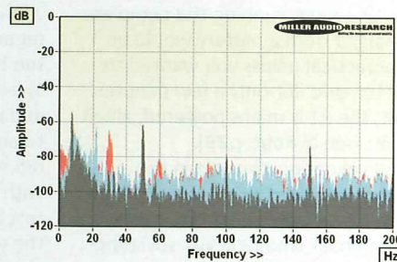
ABOVE: Unweighted bearing rumble from DC-200Hz (black infill) versus silent LP groove (with vacuum hold-down, blue; without, red) re. 1kHz at 5cm/sec
