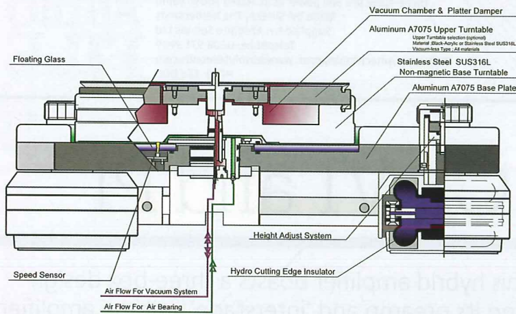
ABOVE: Cutaway diagram illustrating the key layers and components of the Air Force One. The separate AC motor is not included in the drawing, but would sit to the left
