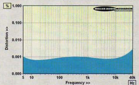
ABOVE: Distortion versus frequency over extended 5Hz-40kHz range (1V output, balanced in/out)
